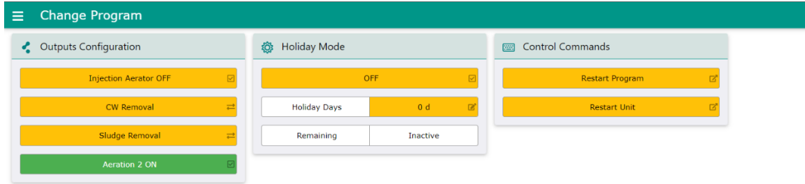
Figure 6: One-Tank SBR program individualization via internal web pages (example)
